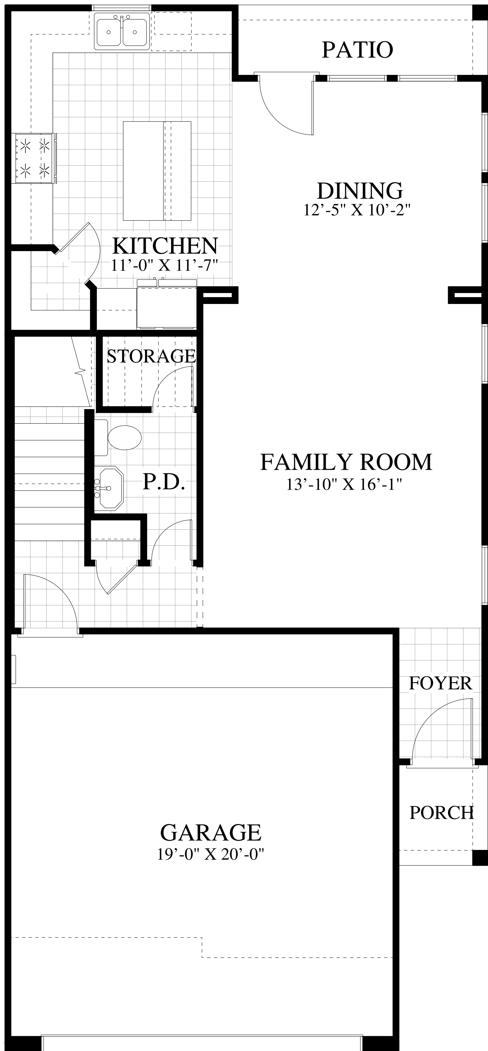
FIRST FLOOR PLAN 737 S.F.
